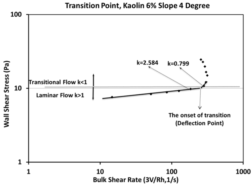
Figure 3 Locus of transition point (Kaolin 6% slope 4^\circ )
