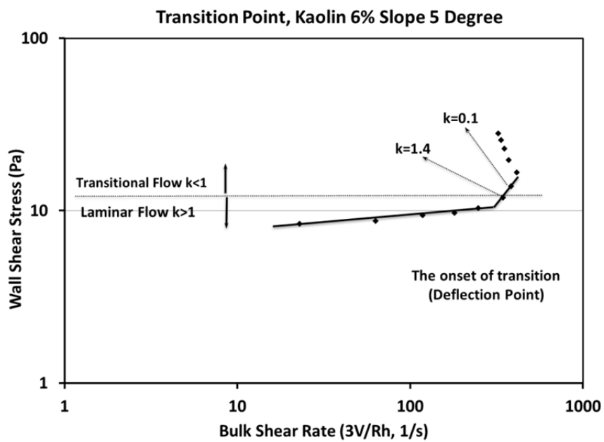
Figure 4 Locus of transition point (Kaolin 6% slope 5^\circ )
